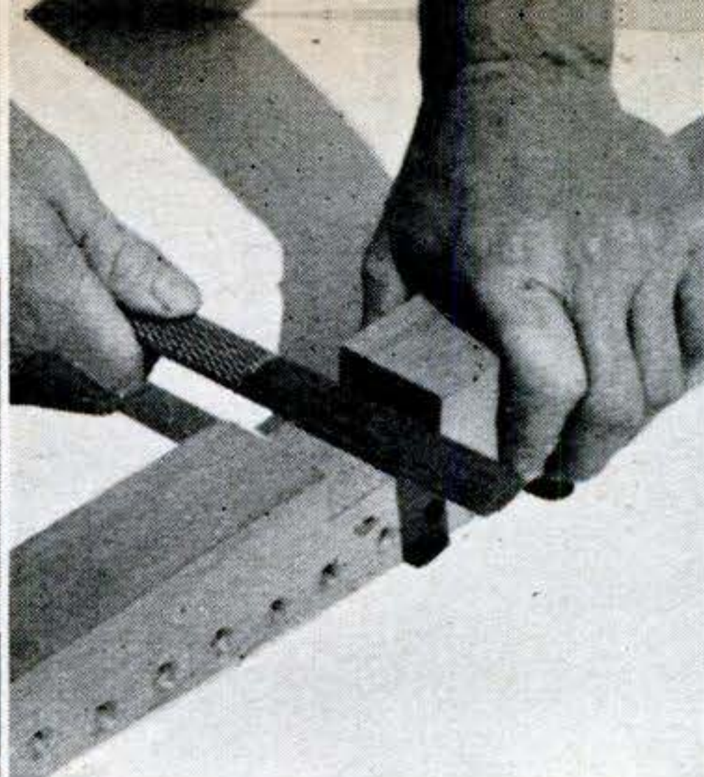
WOOD PARTS are quickly shaped with the half-round shoe rasp. A wood rasp or cabinet rasp is excellent for finishing wood joints, particularly on end grain.
